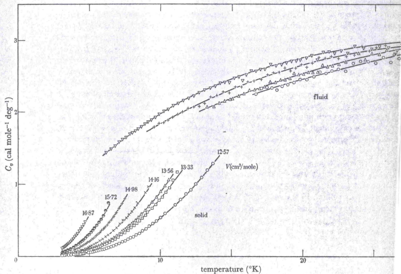
FIGURE 6. The specific heat at constant volume of solid and fluid 3 He at various volumes.
