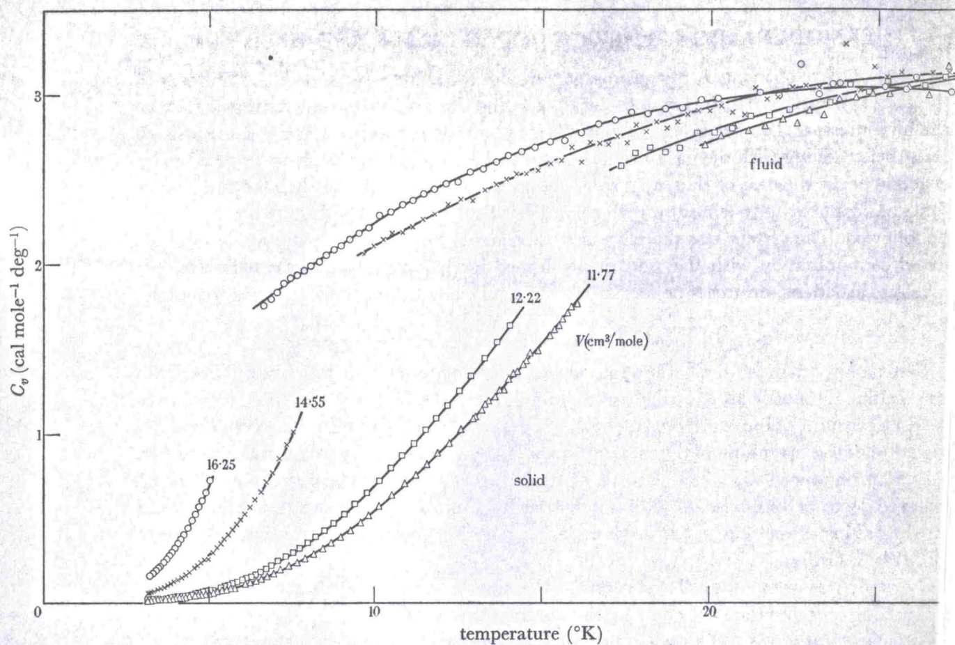
FIGURE 5. The specific heat at constant volume of solid and fluid 4 He at various volumes.
